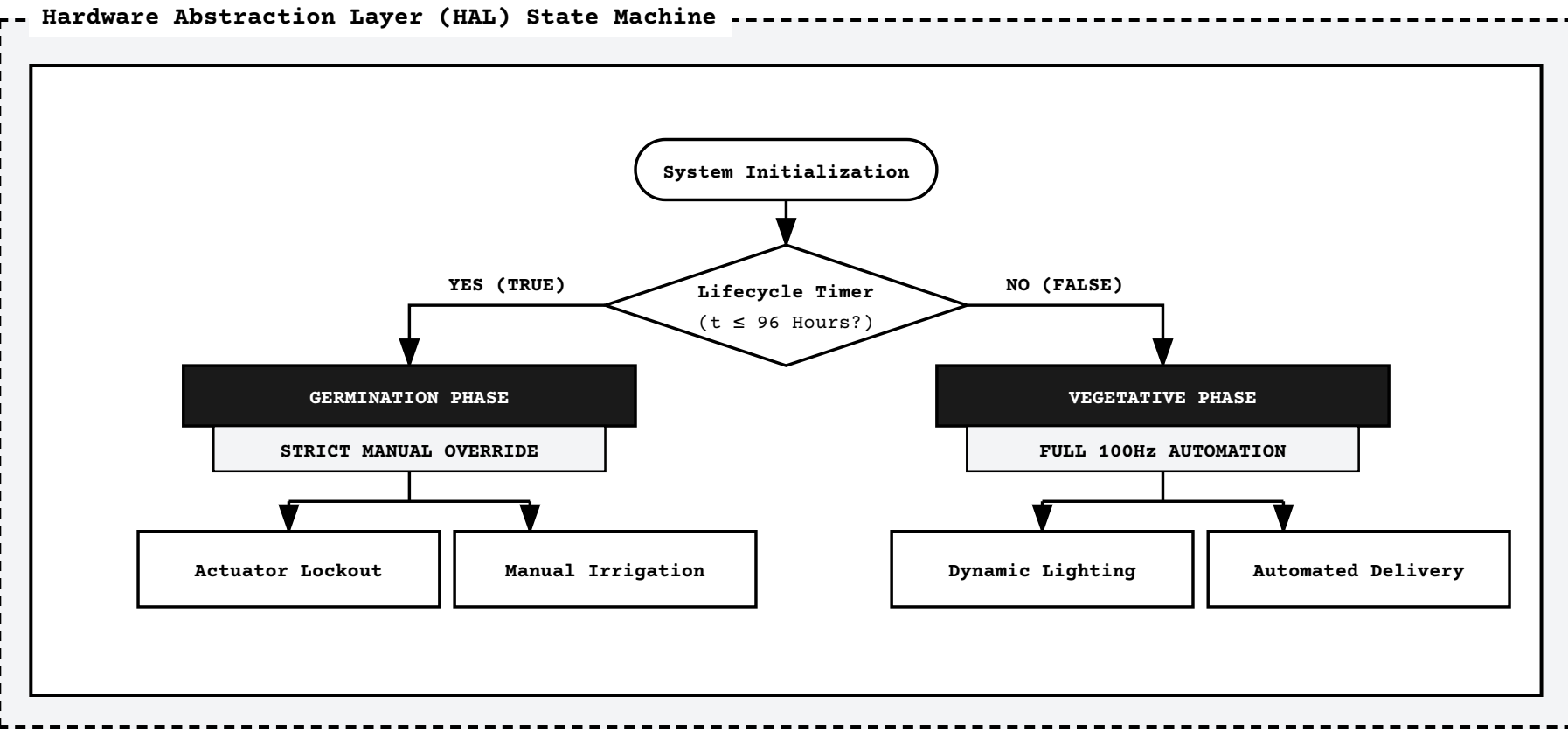
FIGURE 3: SYSTEM OPERATIONAL MODES
